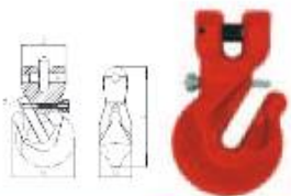
SLR712-SPECIAL TYPE CROOK HOOK WITH SAFETY PIN 带保险销异型羊角抓钩
