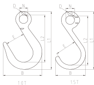
SLR207-ALLOY FORGED LARGE OPENING HOOK 合金钢锻造大开口钩
