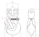
SLR712-SPECIAL TYPE CROOK HOOK WITH SAFETY PIN 带保险销异型羊角钩
