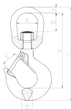
SLR554-FORGED SWIVEL HOOK 旋转钩
