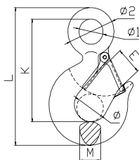
SLR156 - NEW TYPE ALLOY STEEL EYE HOIST HOOK 新型合金钢眼型吊钩
