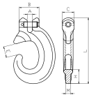
SLR1071-G100 CLEVIS C TYPE HOOK C 型钩
